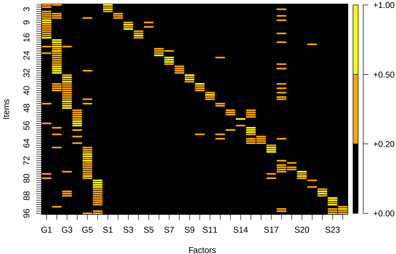
Absolute value of factor loadings (geomin + geomin)
